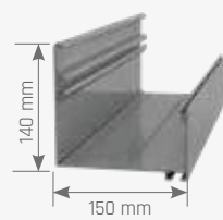
Extruded Frontal Gutter (Water-drain)
